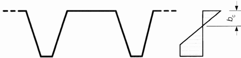
Figure 6.4: Measure b_c for determination of effective width
