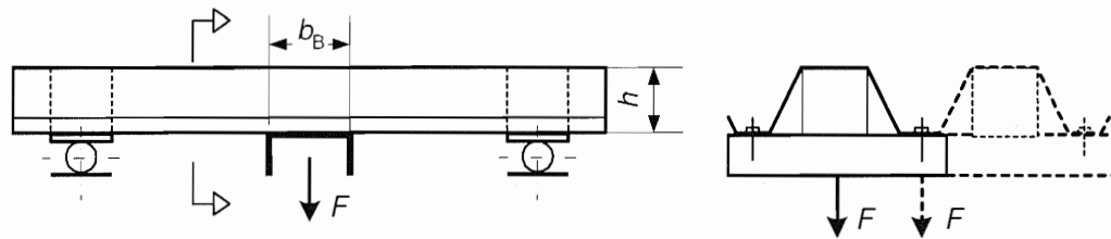
b) Internal support under uplift loading
