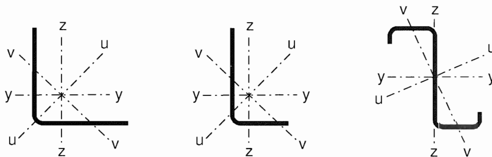
Figure 1.7: Axis convention
