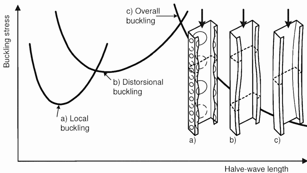
Figure 5.5a: Examples of elastic critical stress for various buckling modes as function of halve-wave length and examples of buckling modes.
