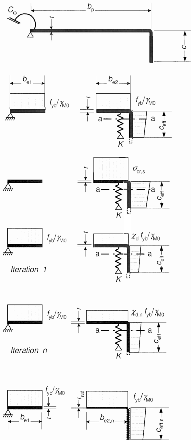
Figure 5.8: Compression resistance of a flange with an edge stiffener
