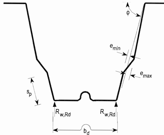
Figure 6.10: Stiffened webs
