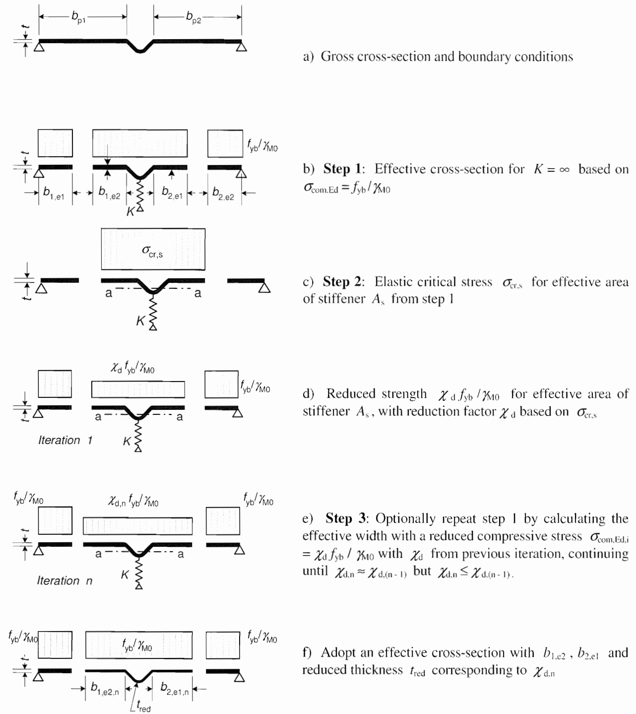
Figure 5.10: Compression resistance of a flange with an intermediate stiffener
