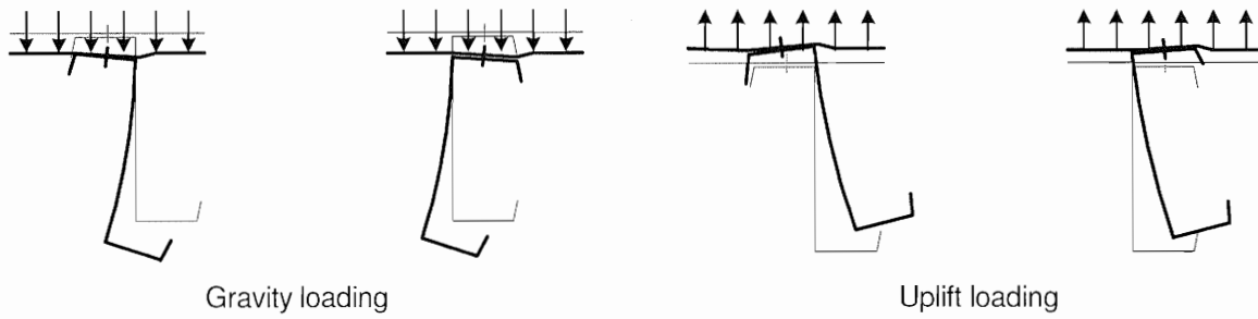
a) Z and C section purlin with upper flange connected to sheeting
