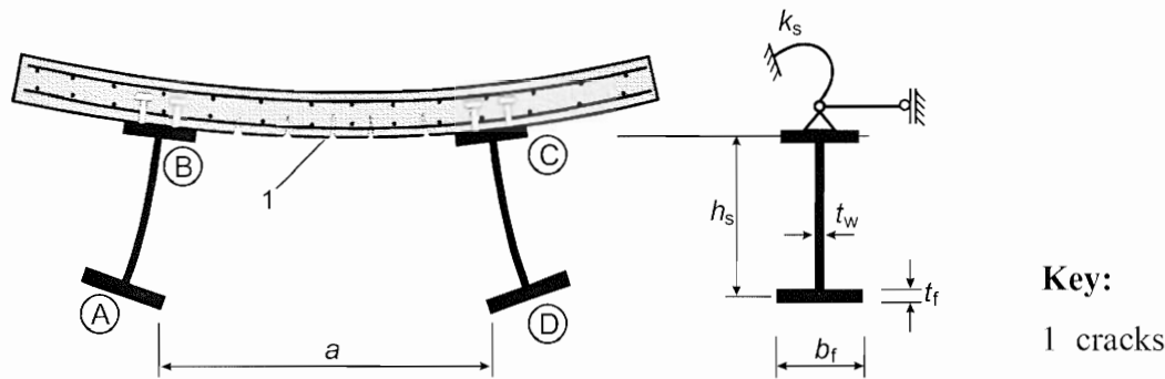
Figure 6.10: U-frame model
