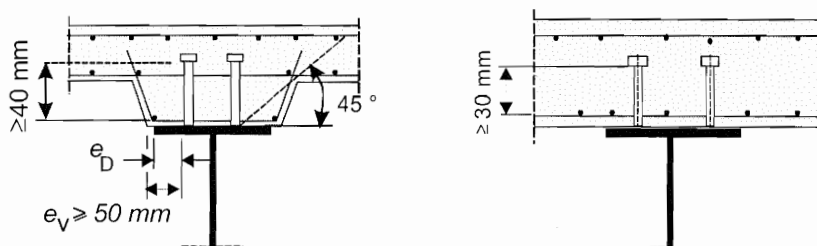
Figure 6.14: Detailing
