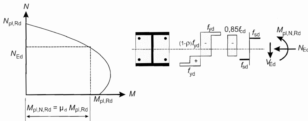
Figure 6.18: Interaction curve for combined compression and uniaxial bending
