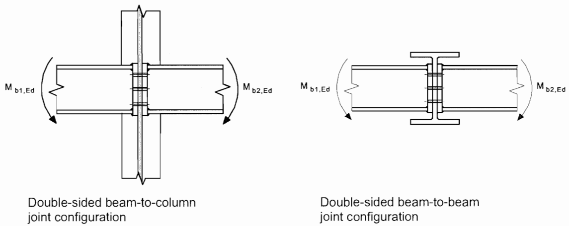
b) Minor-axis joint configurations (to be used only for balanced moments M_{b1,Ed} = M_{b2,Ed} )
