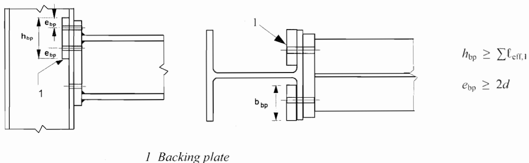
Figure 6.3: Column flange with backing plates
