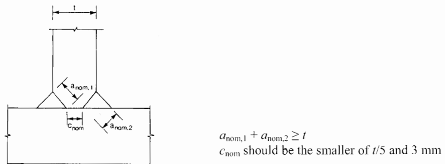
Figure 4.6: Effective full penetration of T-butt welds
