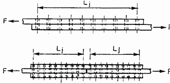
Figure 3.7: Long joints
