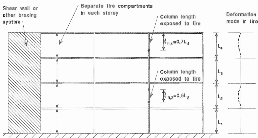
Figure 4.1: Buckling lengths l_{fi} of columns in braced frames
