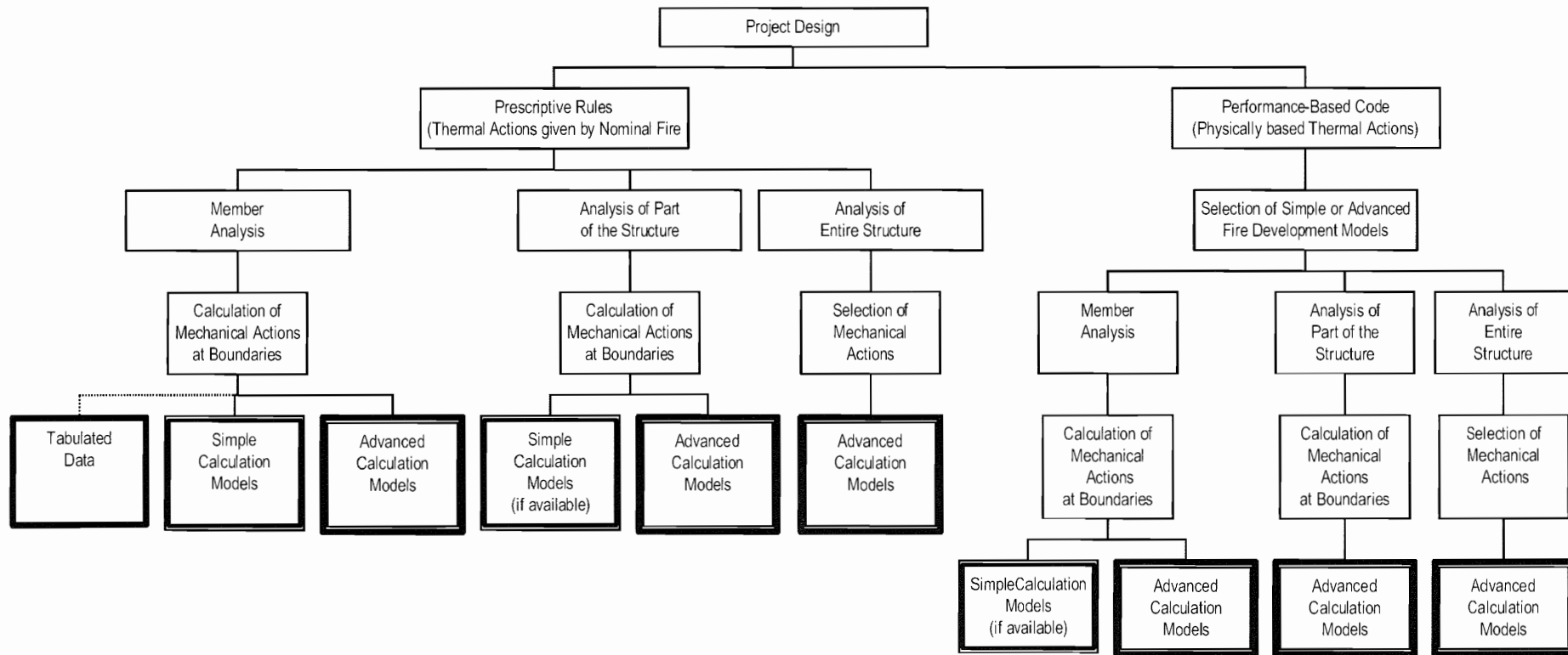
Figure 0.1: Design procedure
