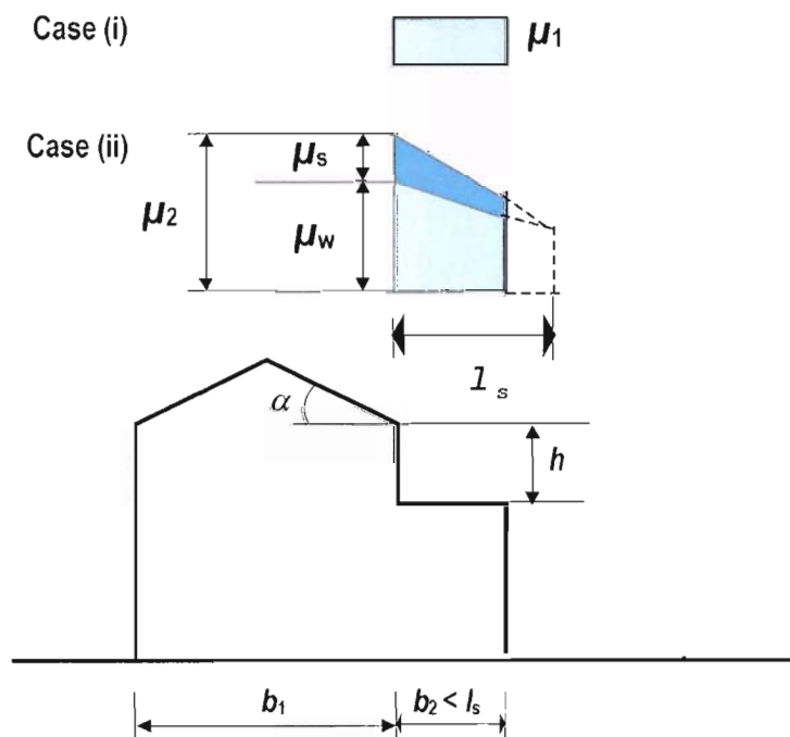
Figure 5.7: Snow load shape coefficients for roofs abutting to taller construction works
