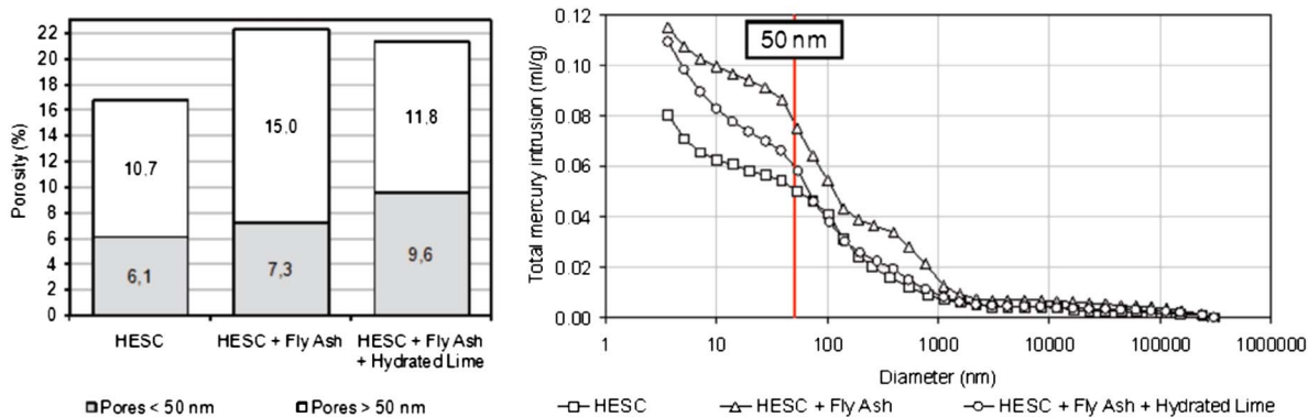
Fig. 10. Porosity and total mercury intrusion in concretes
